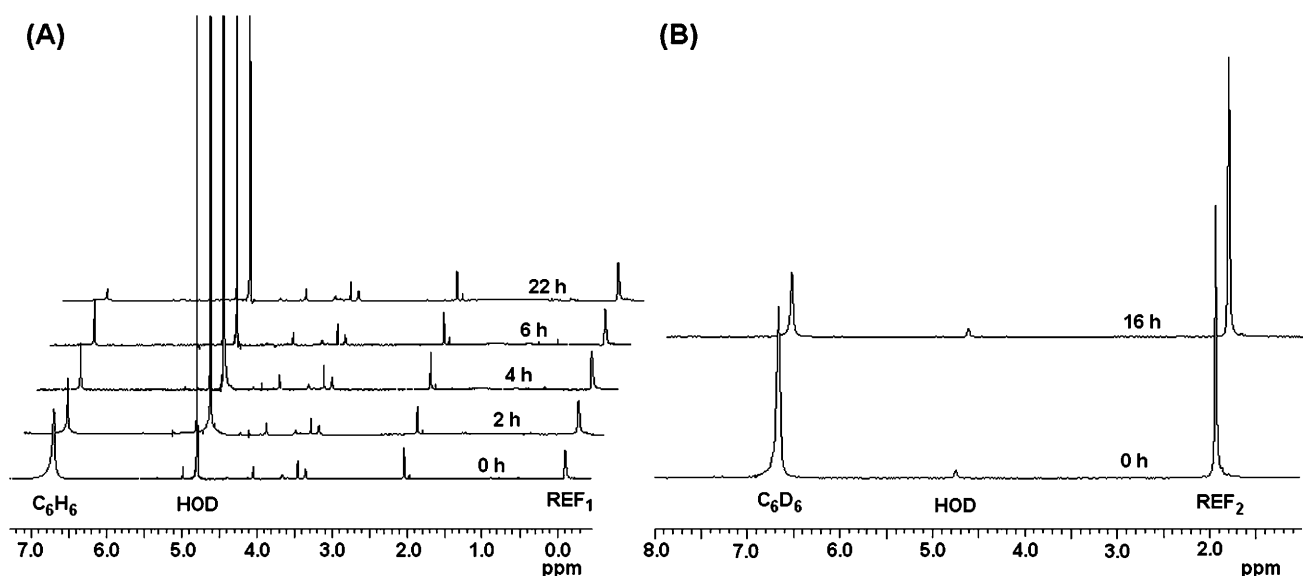
Figure 1. (A) ^1H NMR spectra of a solution of 8a and C_6H_6 in D_2O at 55^\circ C recorded over a period of 22 h. REF_1 (internal standard): poly(dimethylsiloxane). (B) ^2H NMR spectra of solution of 8a and C_6D_6 in H_2O at 55^\circ C recorded after 16 h REF_2 (internal standard): CD_3CN .
